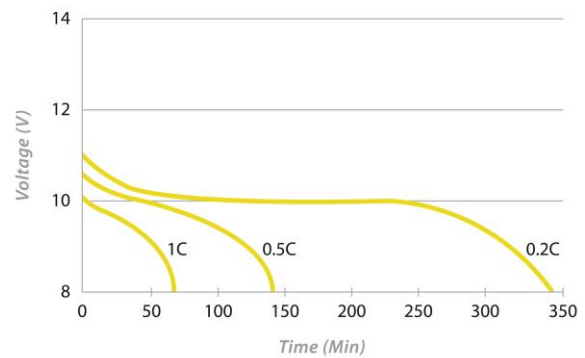
DISCHARGE CHARACTERISTICS
