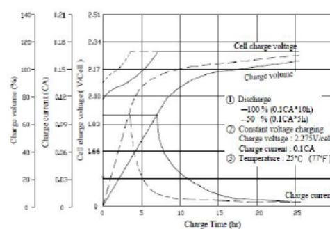
Charging Characteristics for Standby Use
